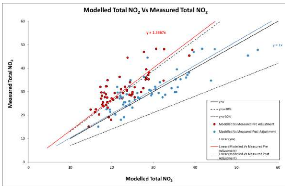
Figure 25 Modelled vs. measured \text{NO}_2 annual mean 2015 before and after adjustment
