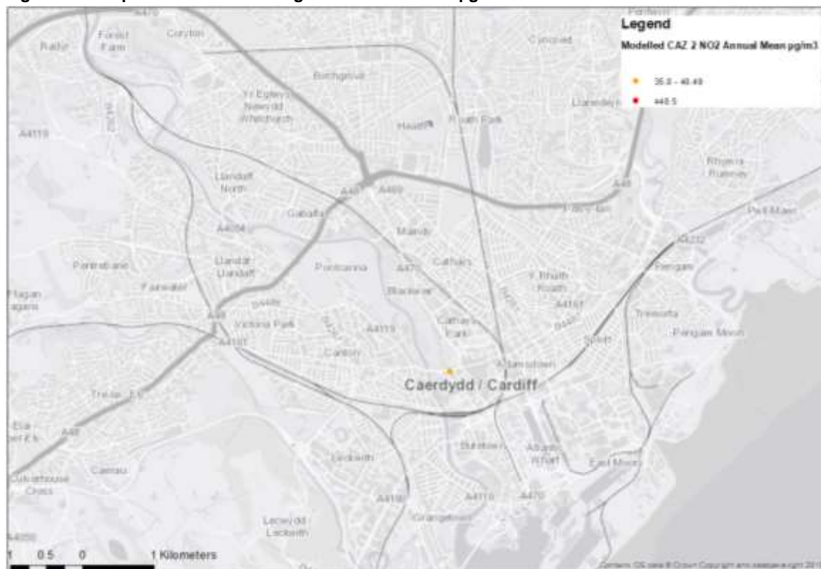
Figure 22 Sampled NO 2 results along the PCM links >35 µg/m 3 for CAZ 2 results in 2021
